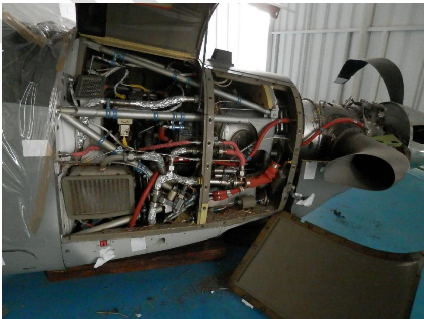
Aircraft powerplant – RH side
